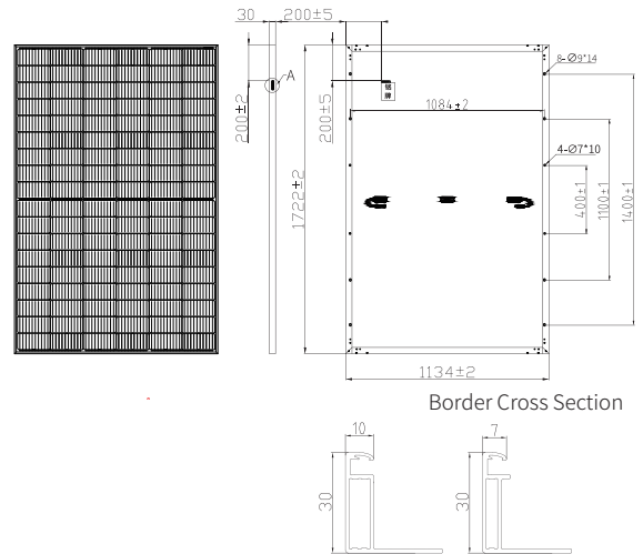
Dimensional drawings (mm)
